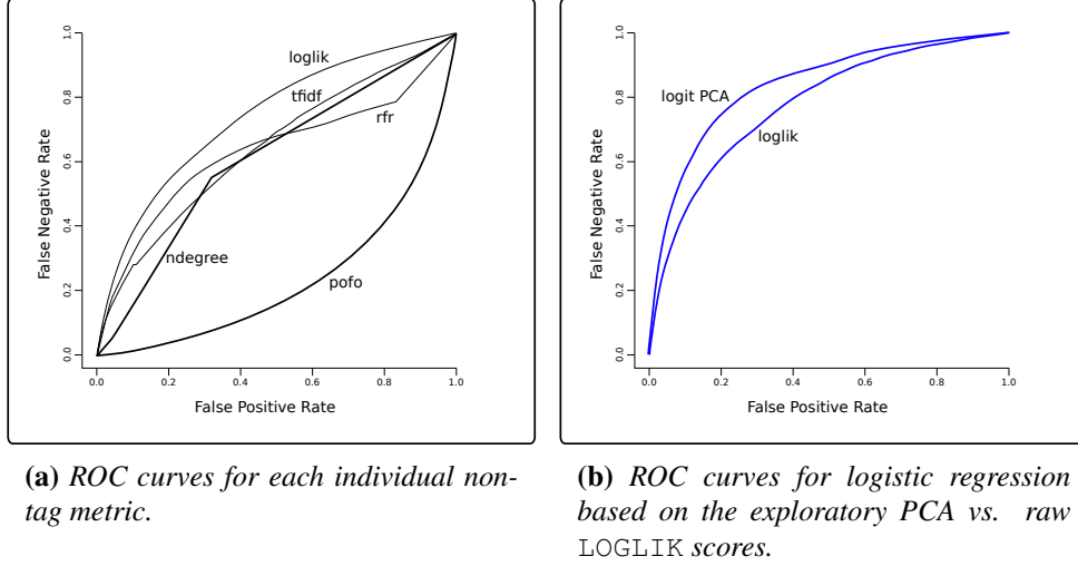
Figure 3: Classifier ROC curves.
