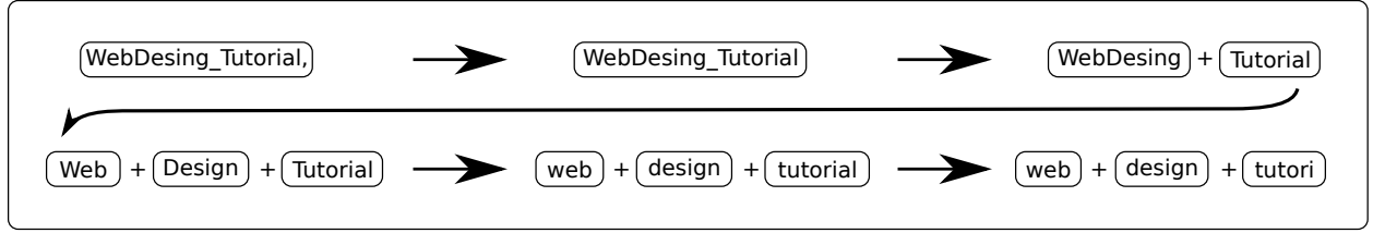
Figure 1: The process of normalising tags.
