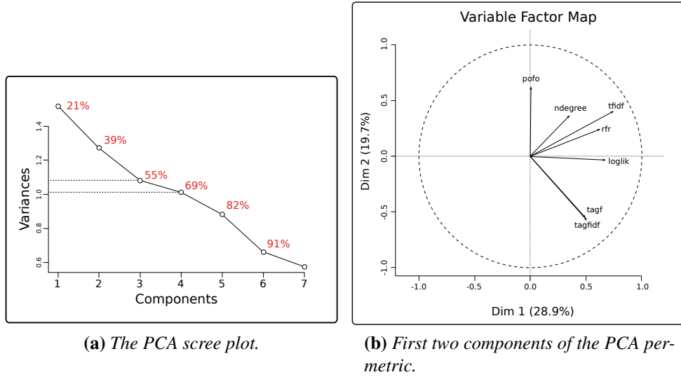
Figure 2: The PCA model parameters.
